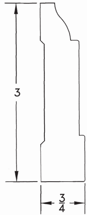
M-1322 \frac{3}{4} \times 3
