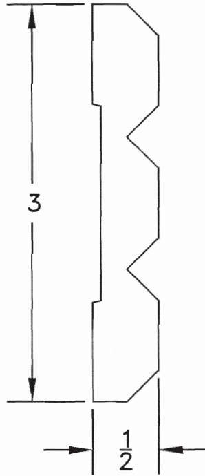
M-1316 \frac{1}{2} \times 3
