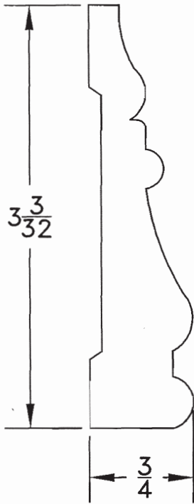
M-1319 \frac{3}{4} \times 3\frac{3}{32}
