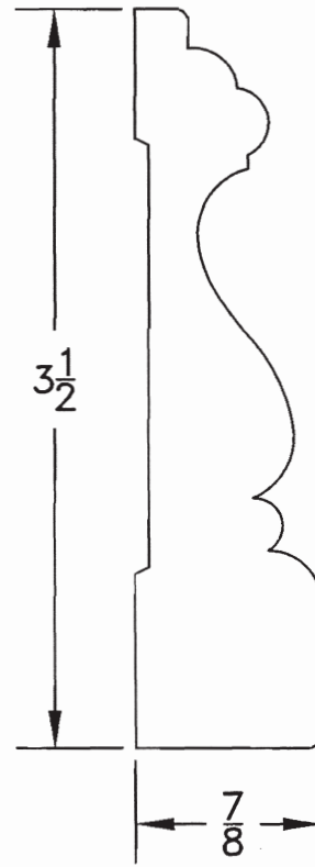
M-1317 \frac{7}{8} \times 3\frac{1}{2}
