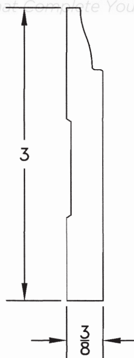
M-233 3/8 x 3
